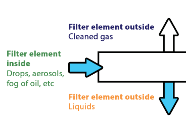
Schematic diagram of coalescing filtration Flow direction from inside to out
